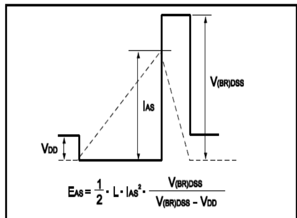
Fig.12 Avalanche Waveform
