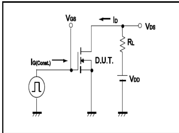
Fig.7 Gate Charge Measurement Circuit
